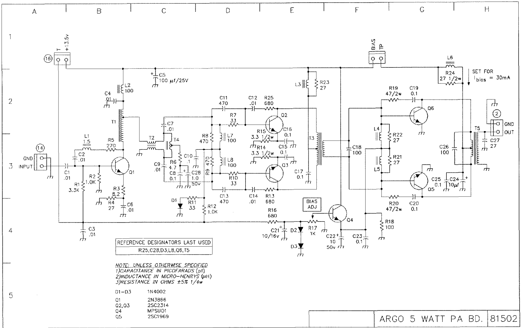
FIGURE 4-8. 5 WATT POWER AMPLIFIER BOARD SCHEMATIC (81502)
