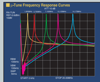
10dB/Div - 2 MHz/Div
