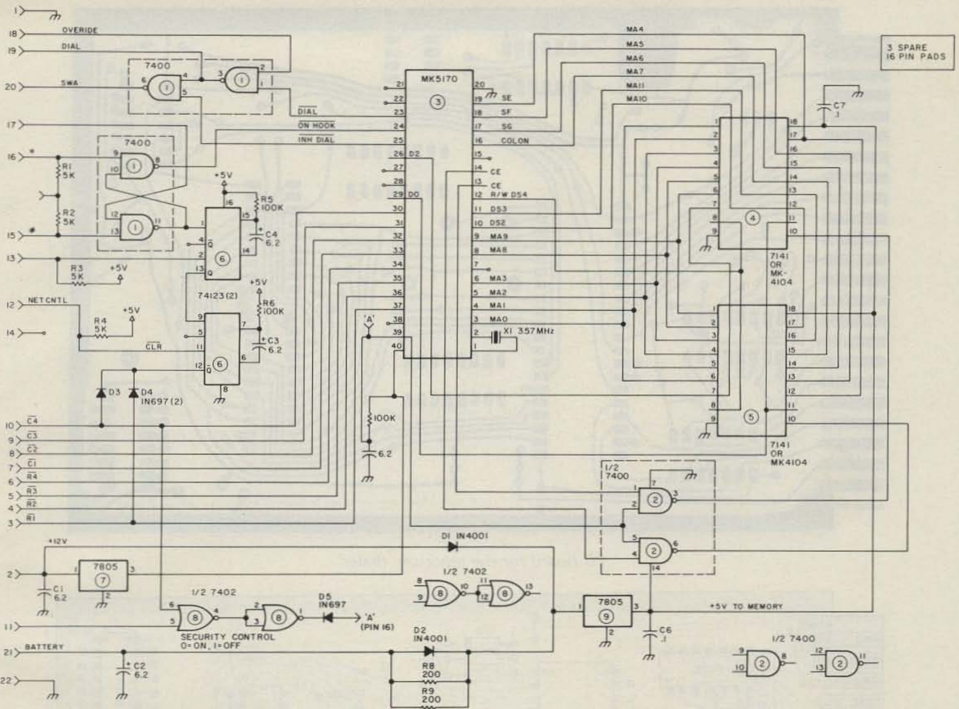
Fig. 2. Circuit diagram for the 100-number system.
