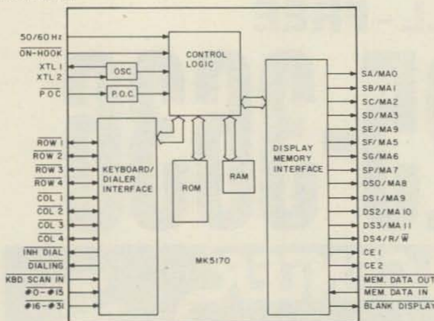
Fig. 1. Pin connections and block diagram.
