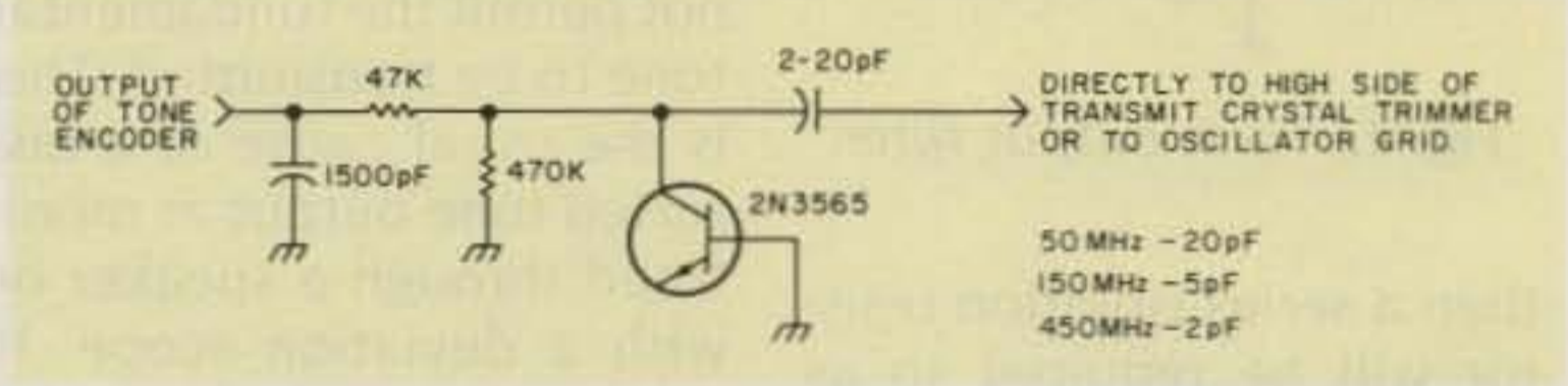
Fig. 2. Schematic of a typical varactor assembly. The collector-base junction of an NPN transistor is used as the varactor. The output of the assembly is connected to the high side of the transmit crystal trimmer. In a tube-type transmitter, the output is often connected to the grid of the oscillator tube. The value of the coupling capacitor changes, depending on the frequency range used. The values shown are approximate and may require adjustment to obtain the proper deviation level.
