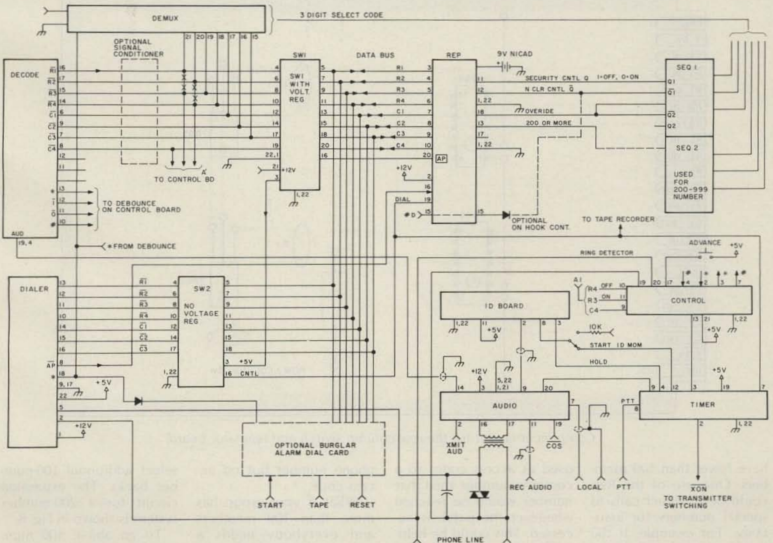
Fig. 5. Basic repeater control system with repertory dialer.
