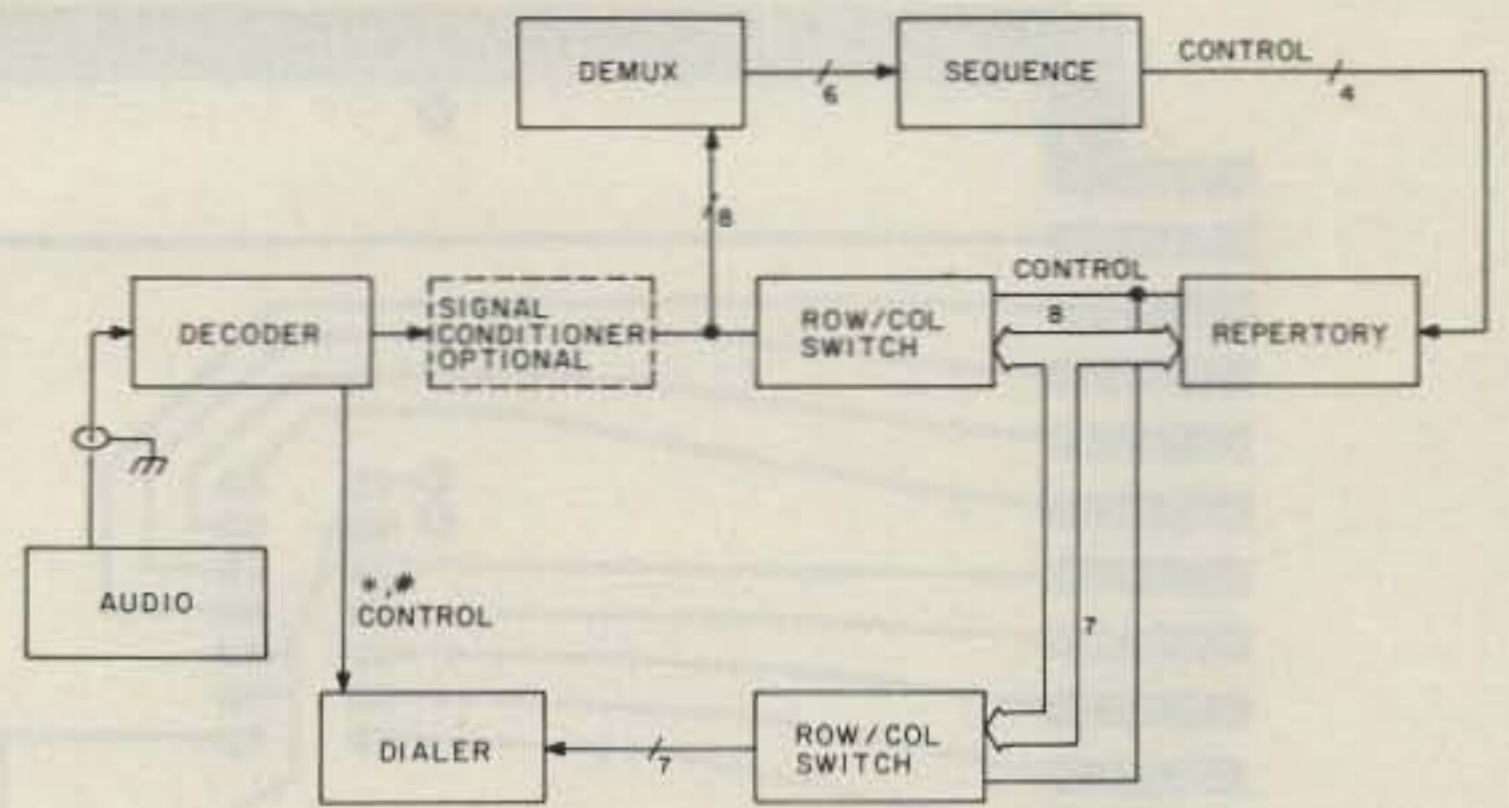
Fig. 4. Repertory connection to phone patch.
