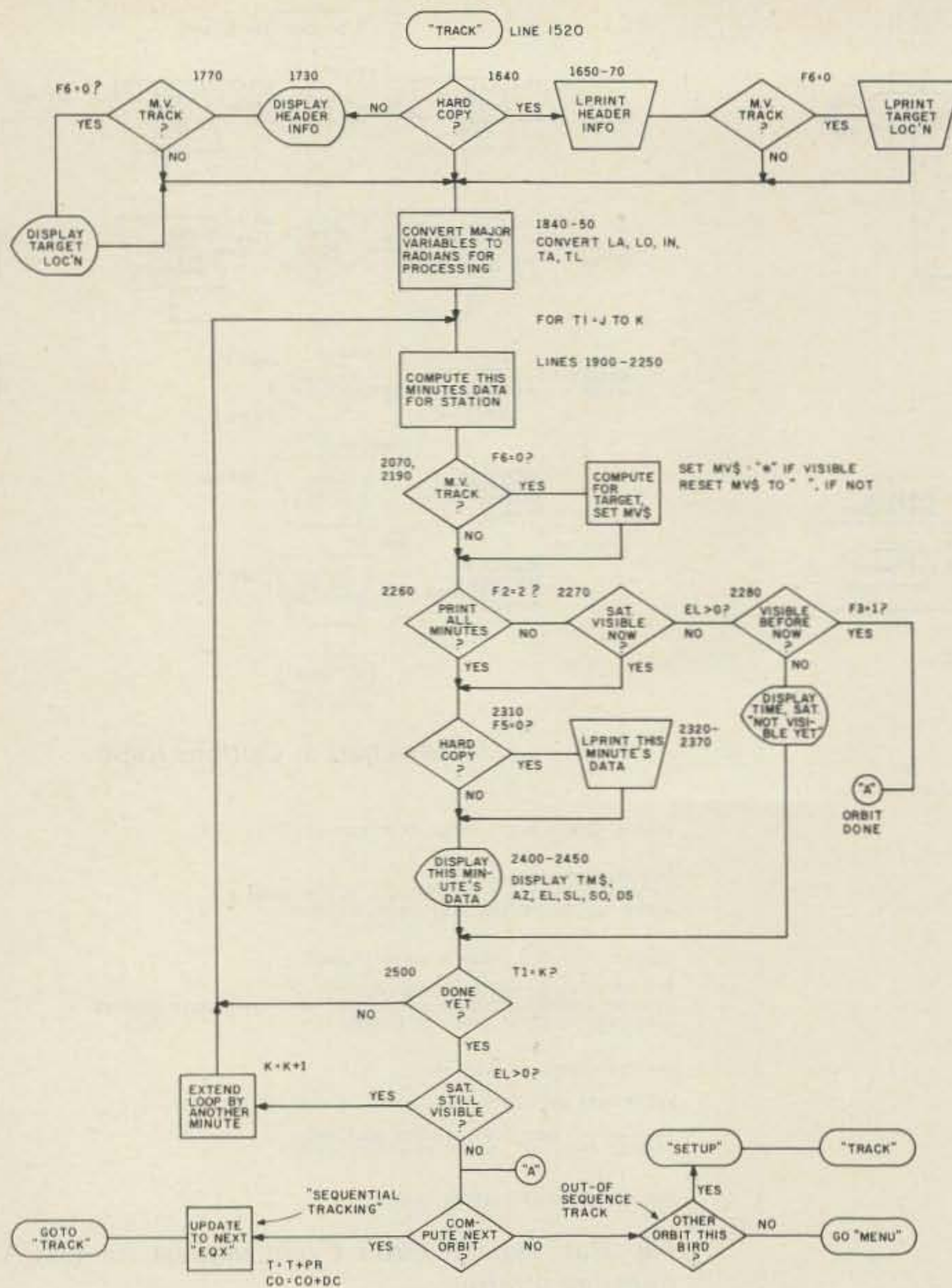
Flowchart 6. Orbit Track logic.
