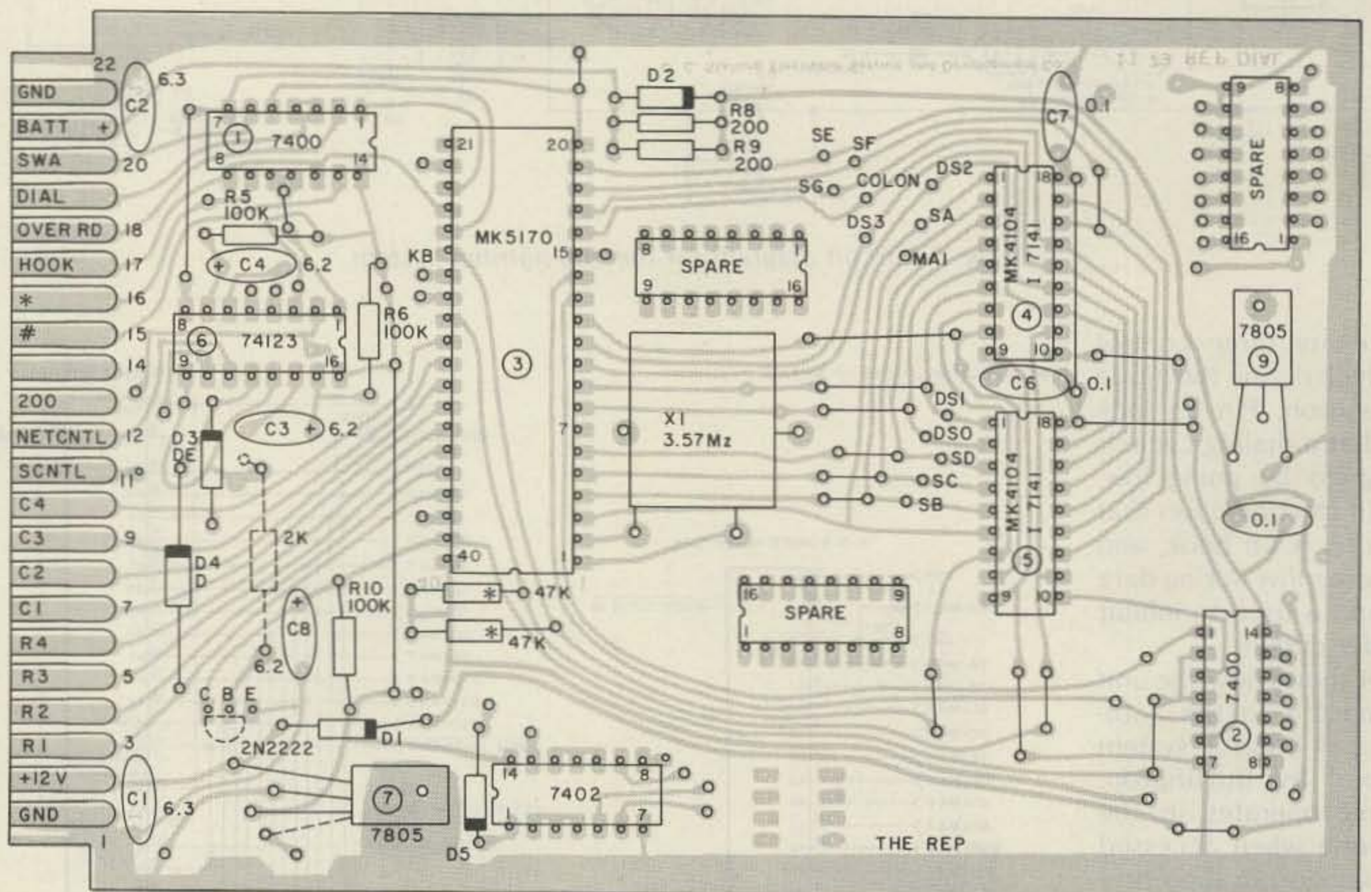
Component layout for repertory dialer.
