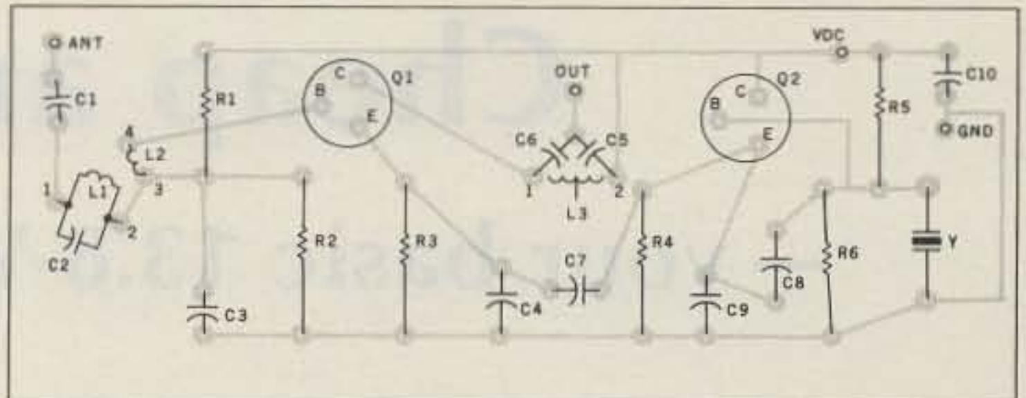
Fig. 3. Parts placement guide (foil side shown).
