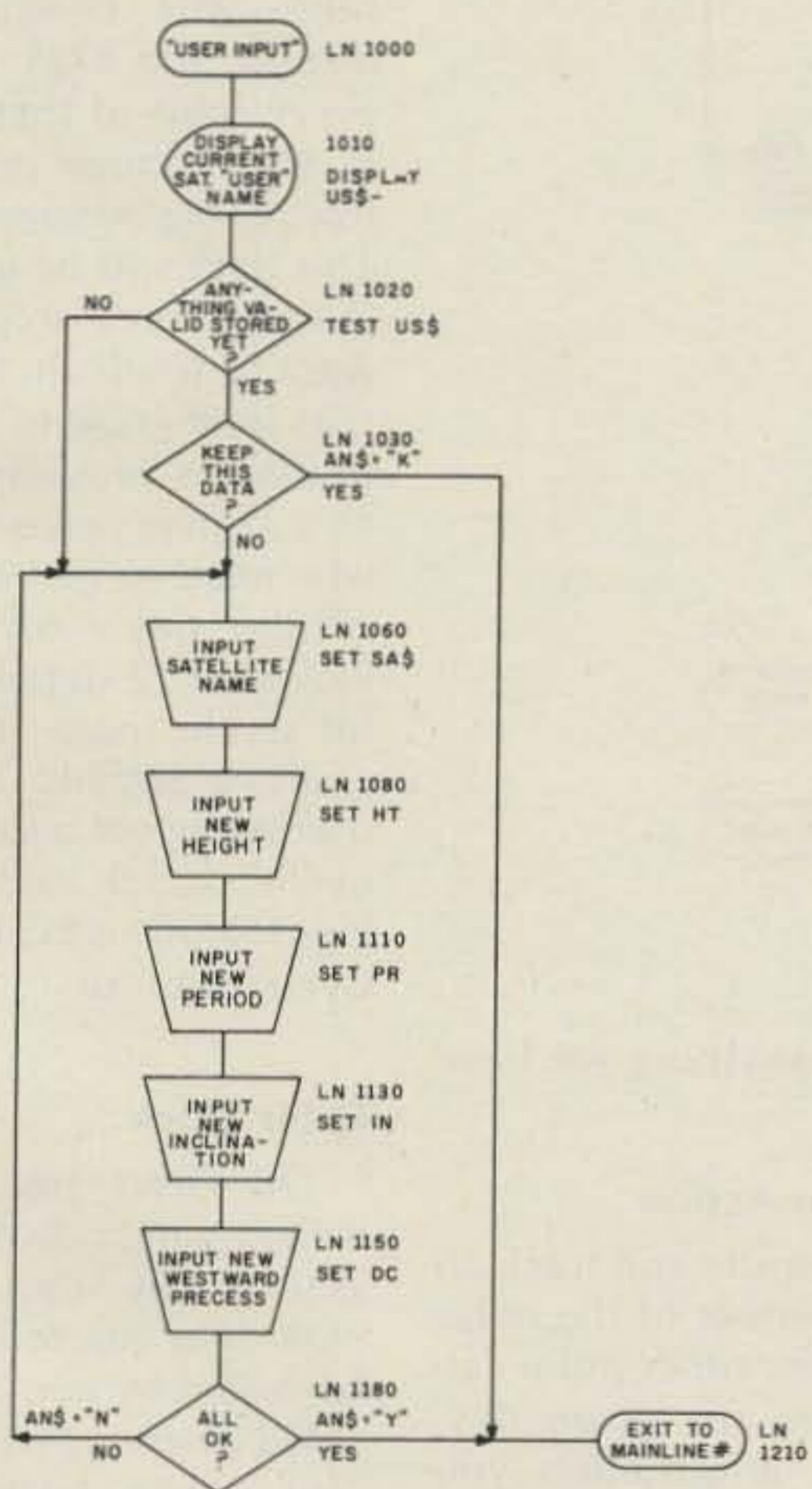
Flowchart 4. User Input Routine logic.
