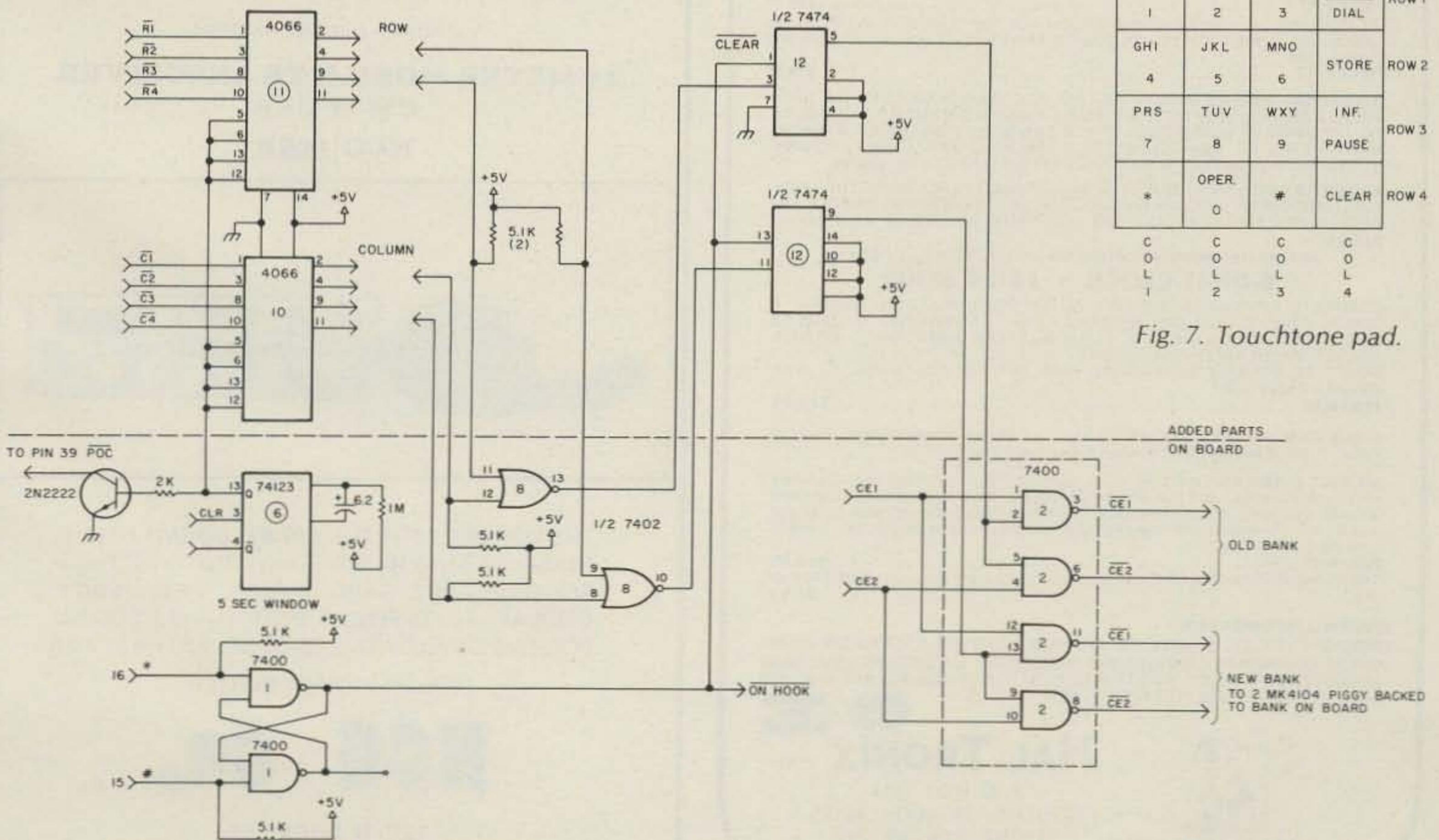
Fig. 8. Expansion circuit for a 200-number system.
