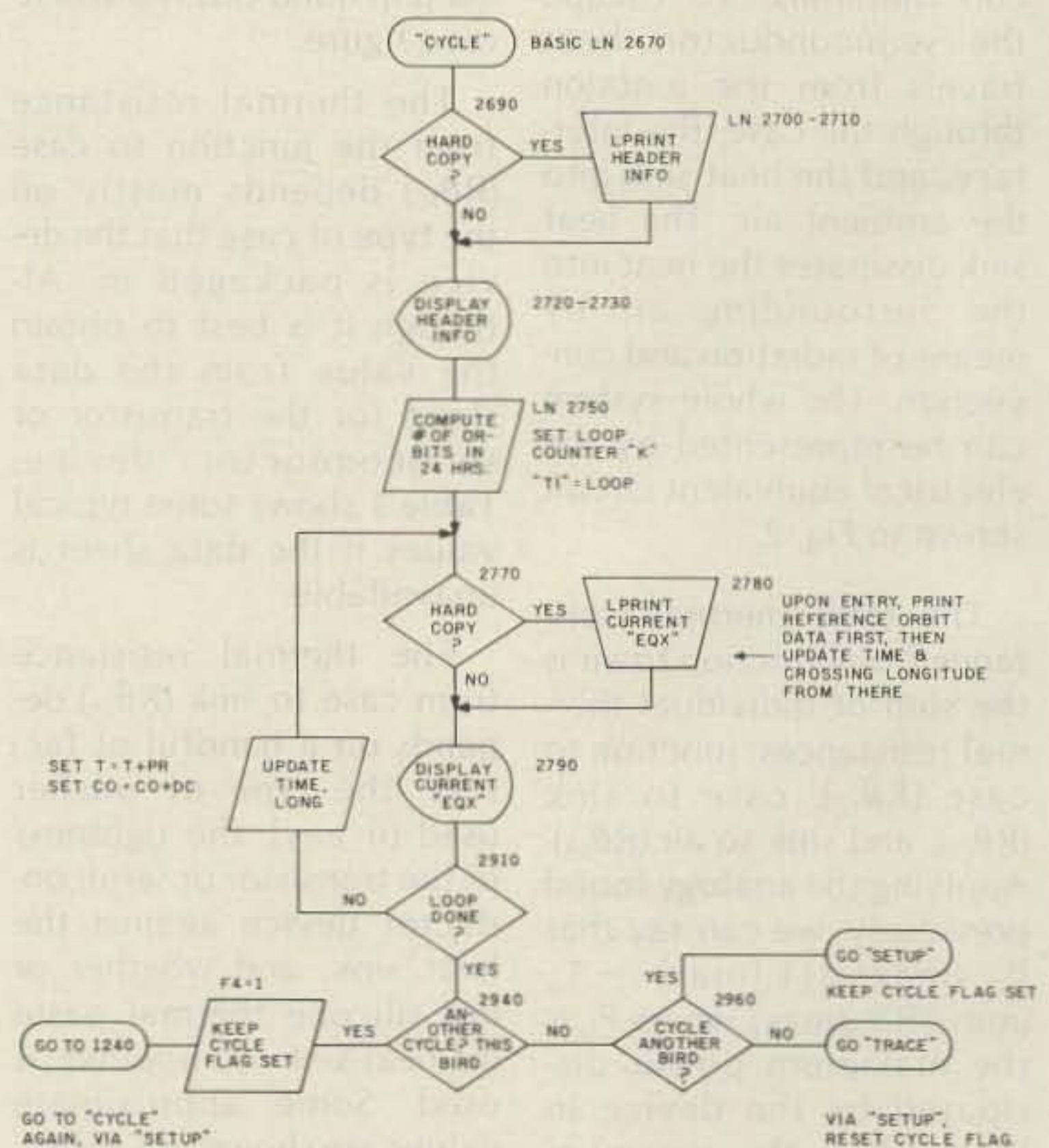
Flowchart 2. Orbit Cycle logic.
