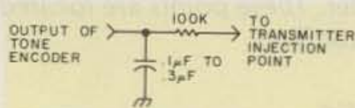
Fig. 4. Tone output filter.
