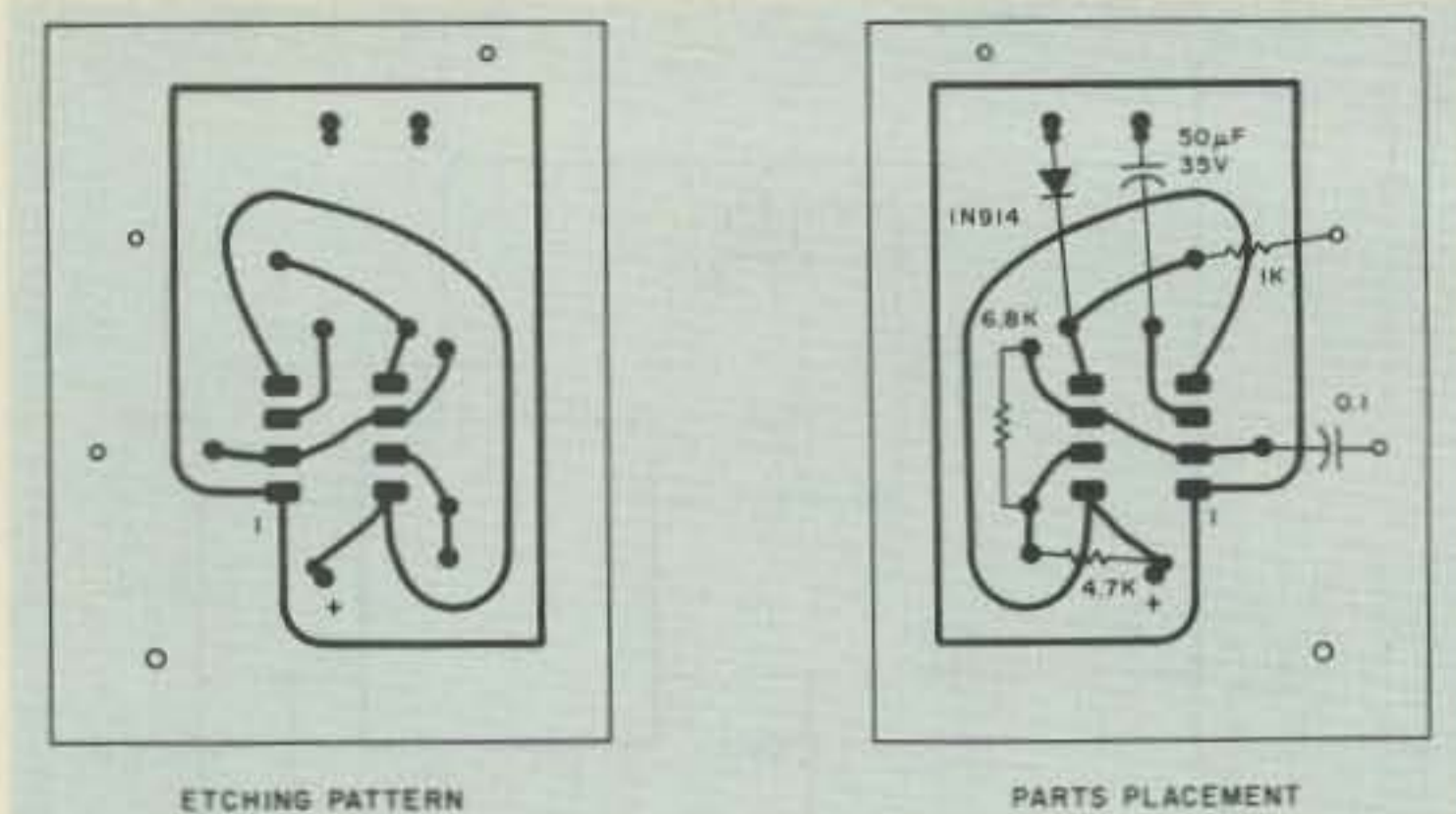
Fig. 3. PCB layout and parts placement.
