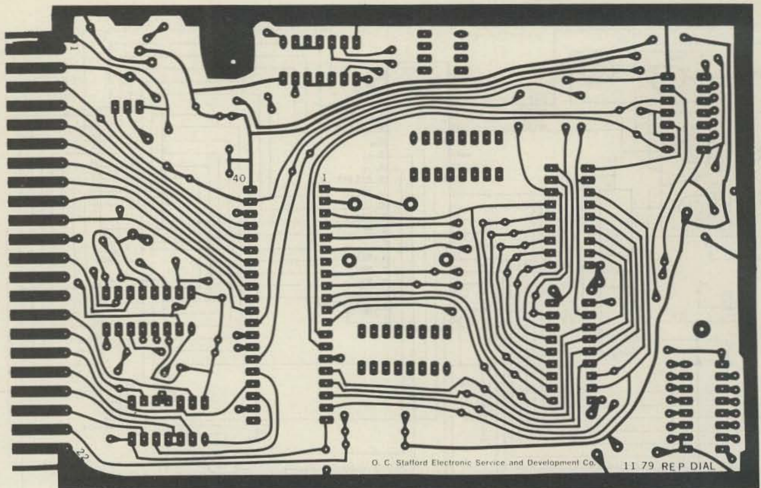
PC board for the repertory dialer.
