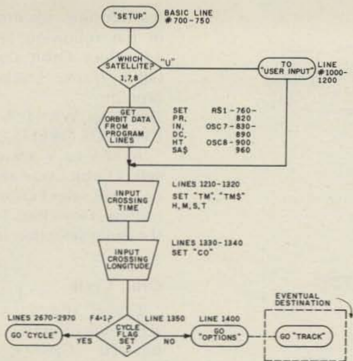
Flowchart 3. Setup logic.
