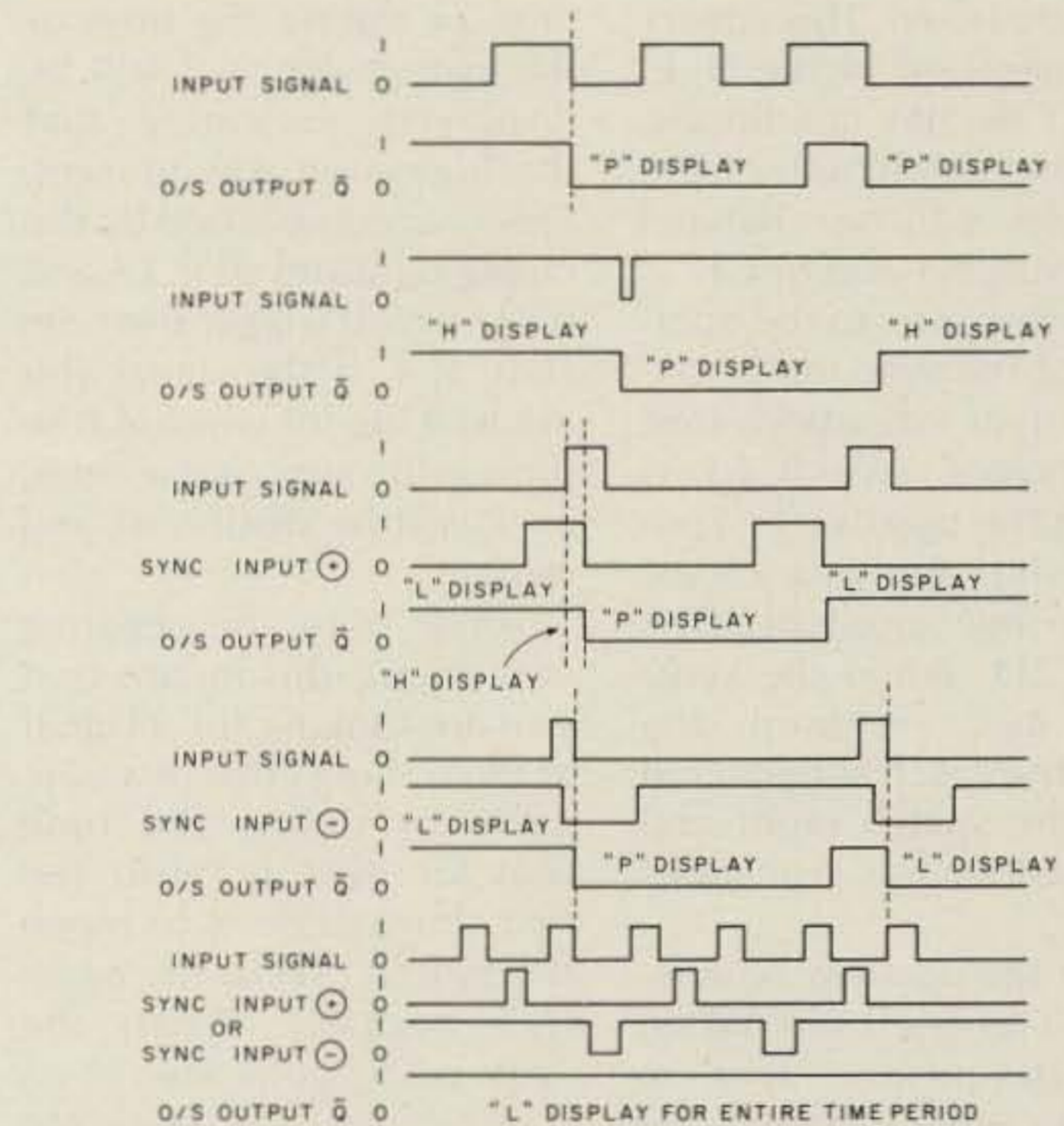
Fig. 2. Timing diagram for logic probe.
