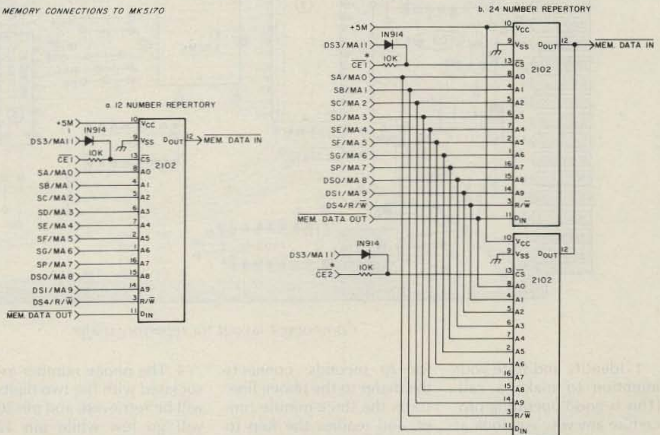
Fig. 3. Memory circuit for a 24-number (or fewer) system. It can be built on header chip and attached to the 18-pin socket.
