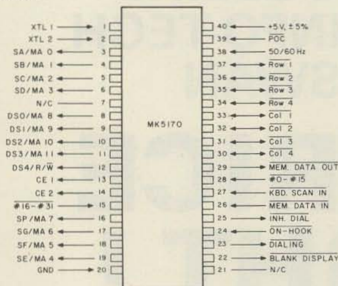
PIN CONNECTIONS
