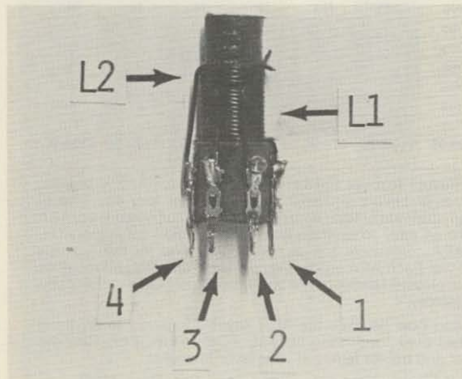
Photo A. Close-up of the L1-L2 inductor. L1 is 12 ccw turns and L2 is 4 ccw turns of #24 enameled wire. L3 is 35 cw turns of #32 enameled wire. All inductors are wound on a 1/4-inch slug-tuned coil form.
