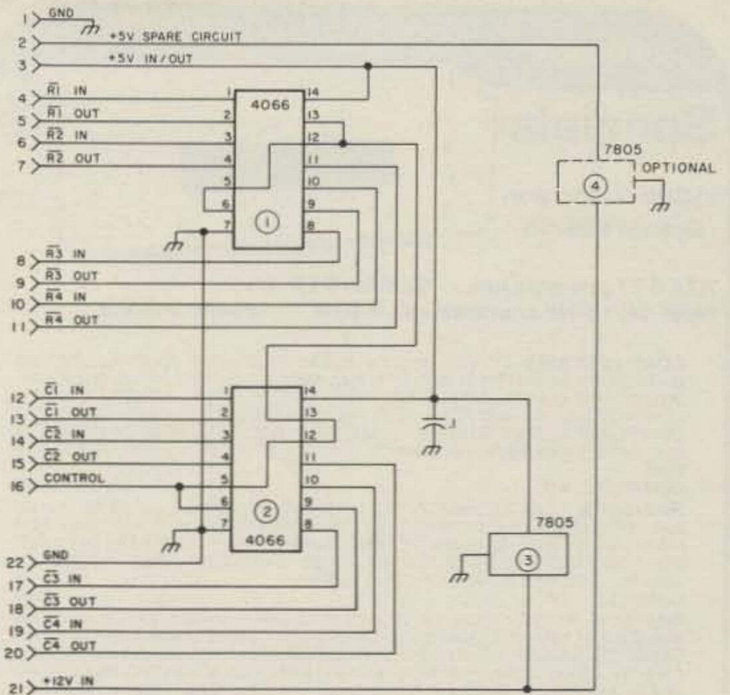
Fig. 6. Row/column switch and regulator board.
