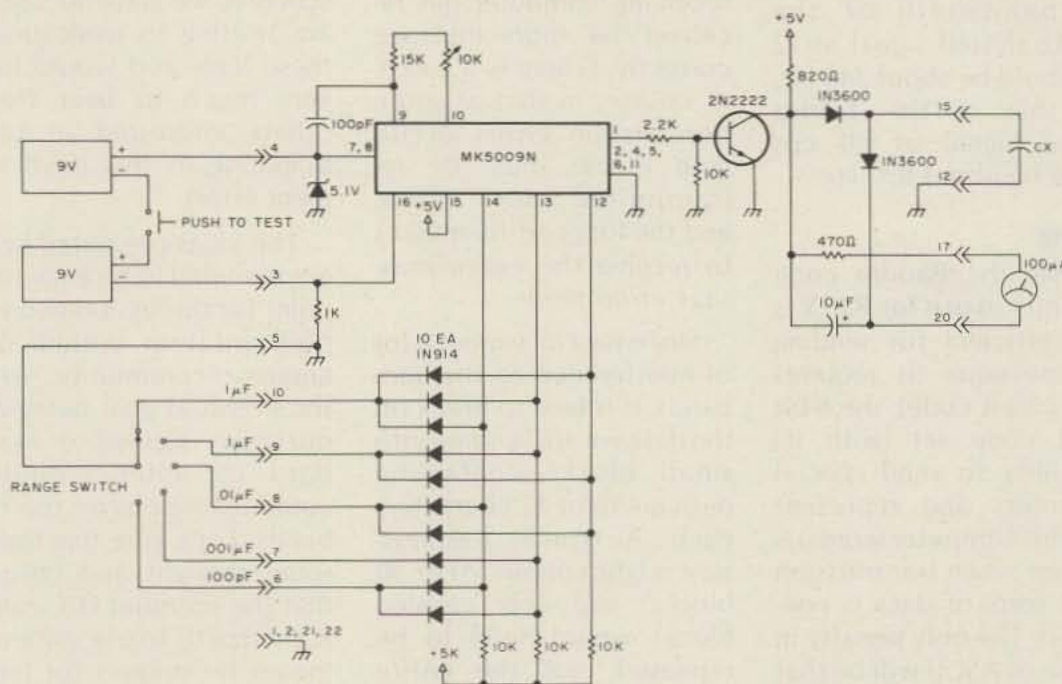
Fig. 1. Capacitor meter schematic.
